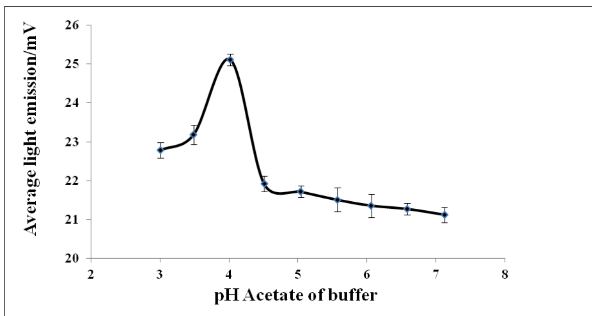
Figure 2. pH effect on ECL.
