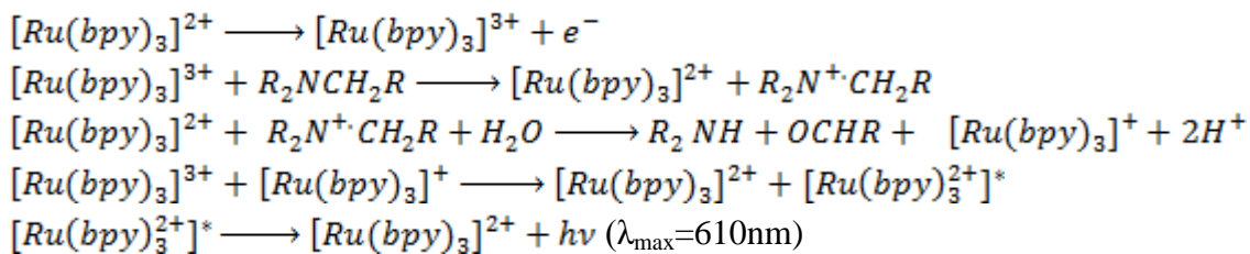
Scheme 3. ECL reaction processes of amine and [Ru(bpy)_3]^{2+} .
