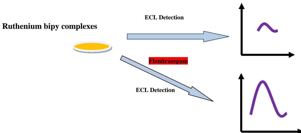
Scheme 1. Detection of Flunitrazepam via ECL.
