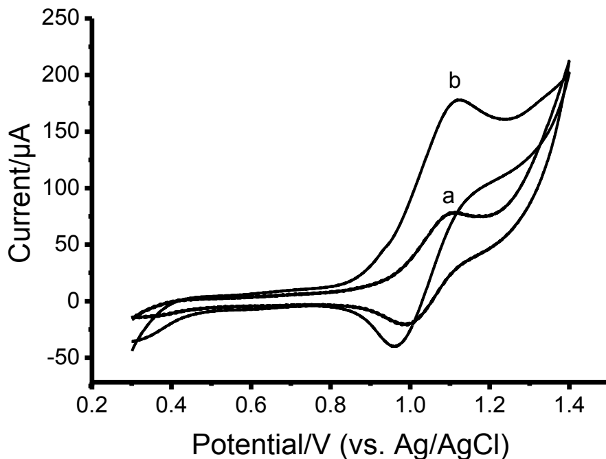
Figure 3. Cyclic voltammograms of the glassy carbon electrode.(a) 1 mM [Ru(bpy)_3]^{2+} in acetate buffer pH 4; (b) 2000ng/mL of Flunitrazepam in 1 mM [Ru(bpy)_3]^{2+} with 1 mM acetate buffer at pH 4 both acquired at scan rate 100 mV/s.
