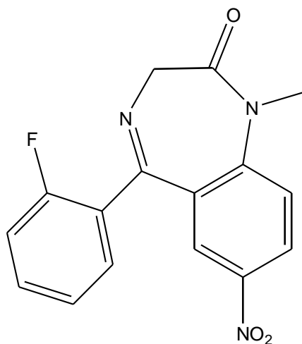
Figure 1. Structure of Flunitrazepam
