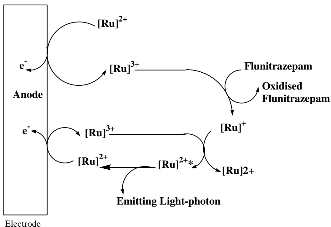
Scheme 2. Emission of light with Flunitrazepam via ECL.
