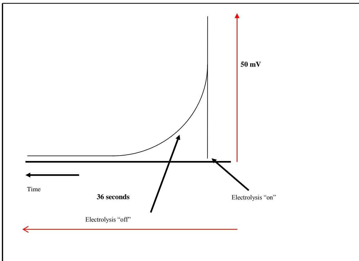
Figure 5. Typical response of ECL transient (signal vs. time) obtained under a single stepped potential electrolysis for 2000 ng/mL of Flunitrazepam in 1mM [Ru(bpy)_3]^{2+} with 1 mM acetate buffer at pH 4.
