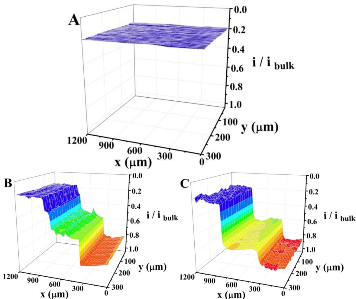
Figure 4. Topographic SECM images of the enamel surface after etching in mineral water (control experiment) (A), 20 \text{mmol L}^{-1} citric acid solution pH 2.2 (B) and 80 \text{mmol L}^{-1} HCl solution pH 1.2 (C). Experiments carried out with a Pt tip ( r = 10 \mu\text{m} and \text{RG} = 10 ) in 15 \text{mmol L}^{-1} \text{K}_3[\text{Fe}(\text{CN})_6] + 0.1 \text{mol L}^{-1} KCl solution. E_{\text{tip}} = -100 \text{ mV} , and v = 20 \mu\text{m s}^{-1} .
