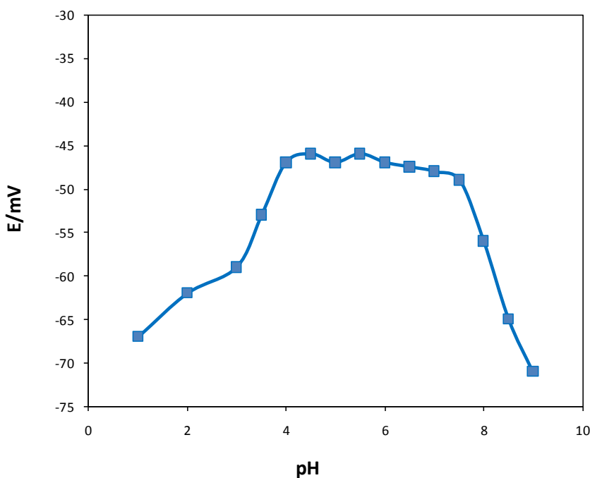
Figure 3. Applicable pH of the electrodes in the test solution of 1.0 \times 10^{-4} M
