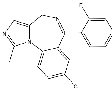
Figure 1. Chemical structure of Midazolam
