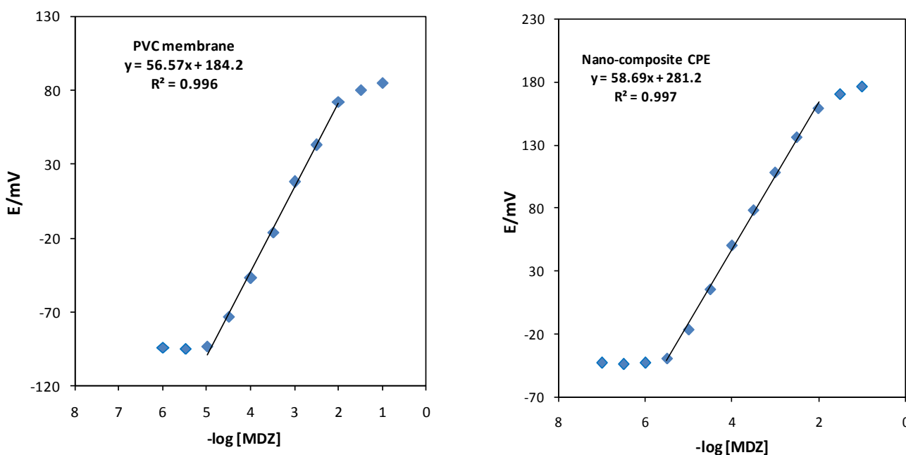
Figure 2. Calibration curves of CPE and PVC membrane electrode. The results are based on 5 replicate measurements.
